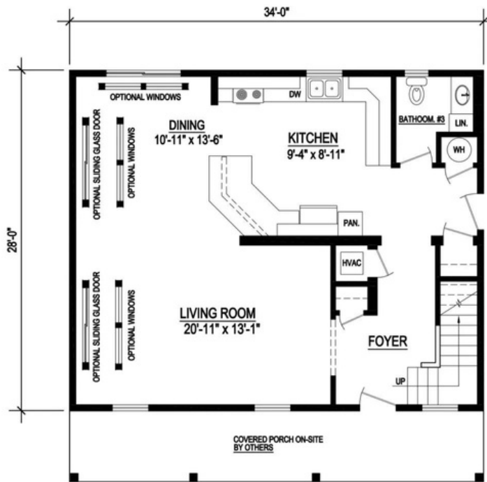
1st LEVEL
